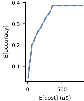
SimpleQA
