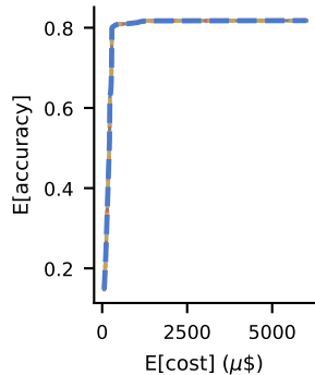
MATH
