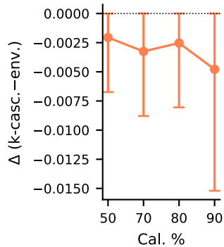
MATH
