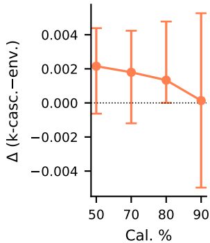
SimpleQA
