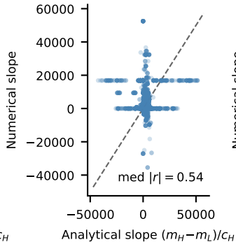
SimpleQA
