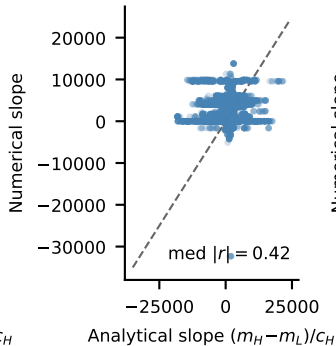
MATH
