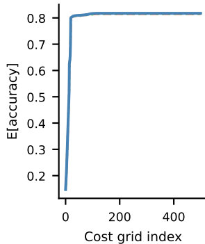
MATH
