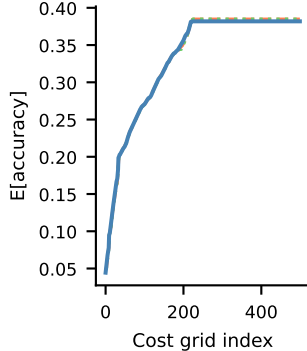
SimpleQA
