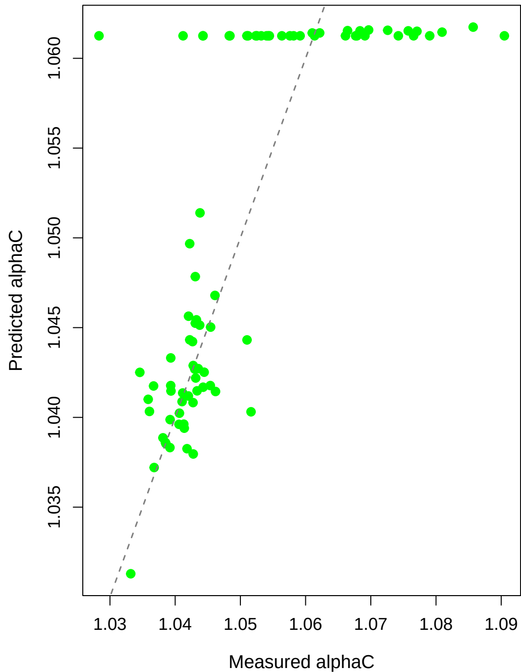
PLS LOO Performance (comp = 5, R^2 = 0.540 , RMSE = 0.009)
