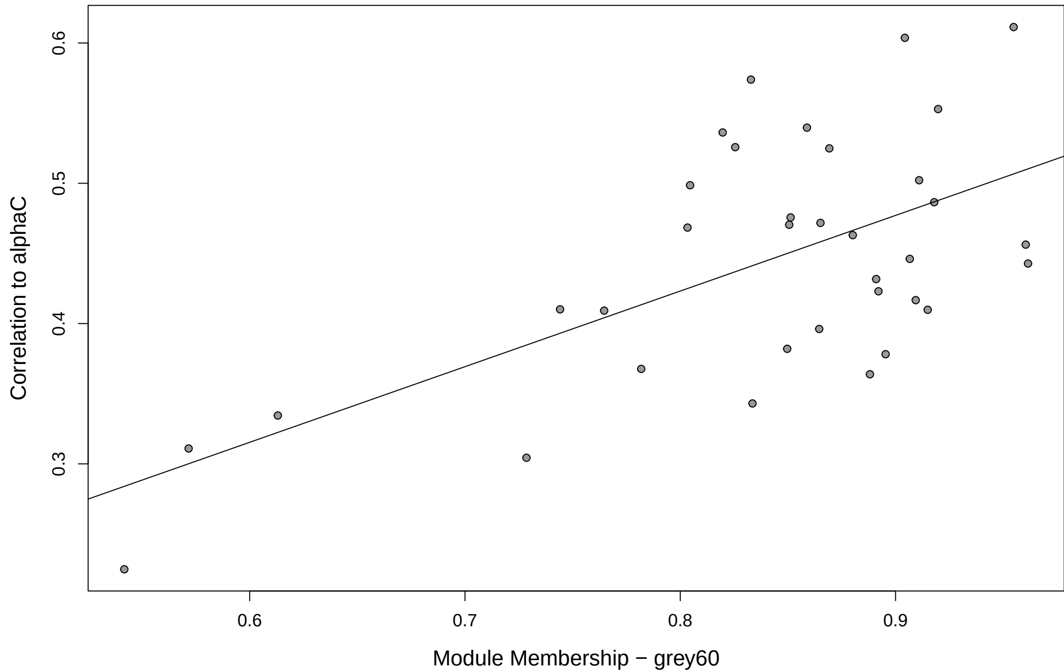
Module Membership vs. Trait Significance (Module: grey60 | Trait: alphaC) cor=0.62, p=7.1e-05
