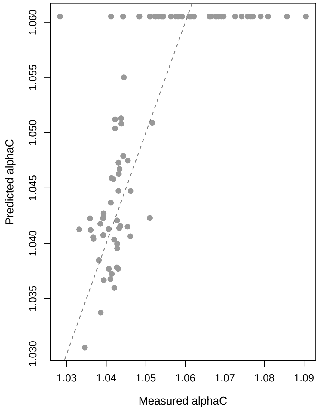
PLS LOO Performance (comp = 5, R^2 = 0.507 , RMSE = 0.010)
