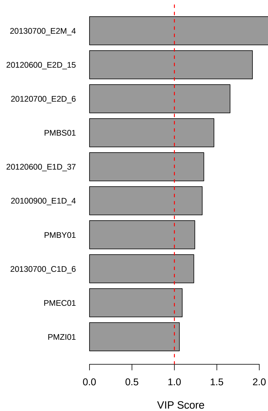
Predictors with VIP > 1 in Module: grey60 (Predicting \alpha C )
