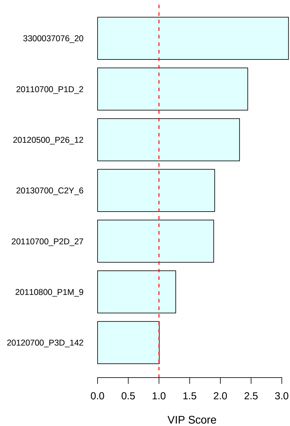
Predictors with VIP > 1 in Module: lightcyan (Predicting \alpha_C )
