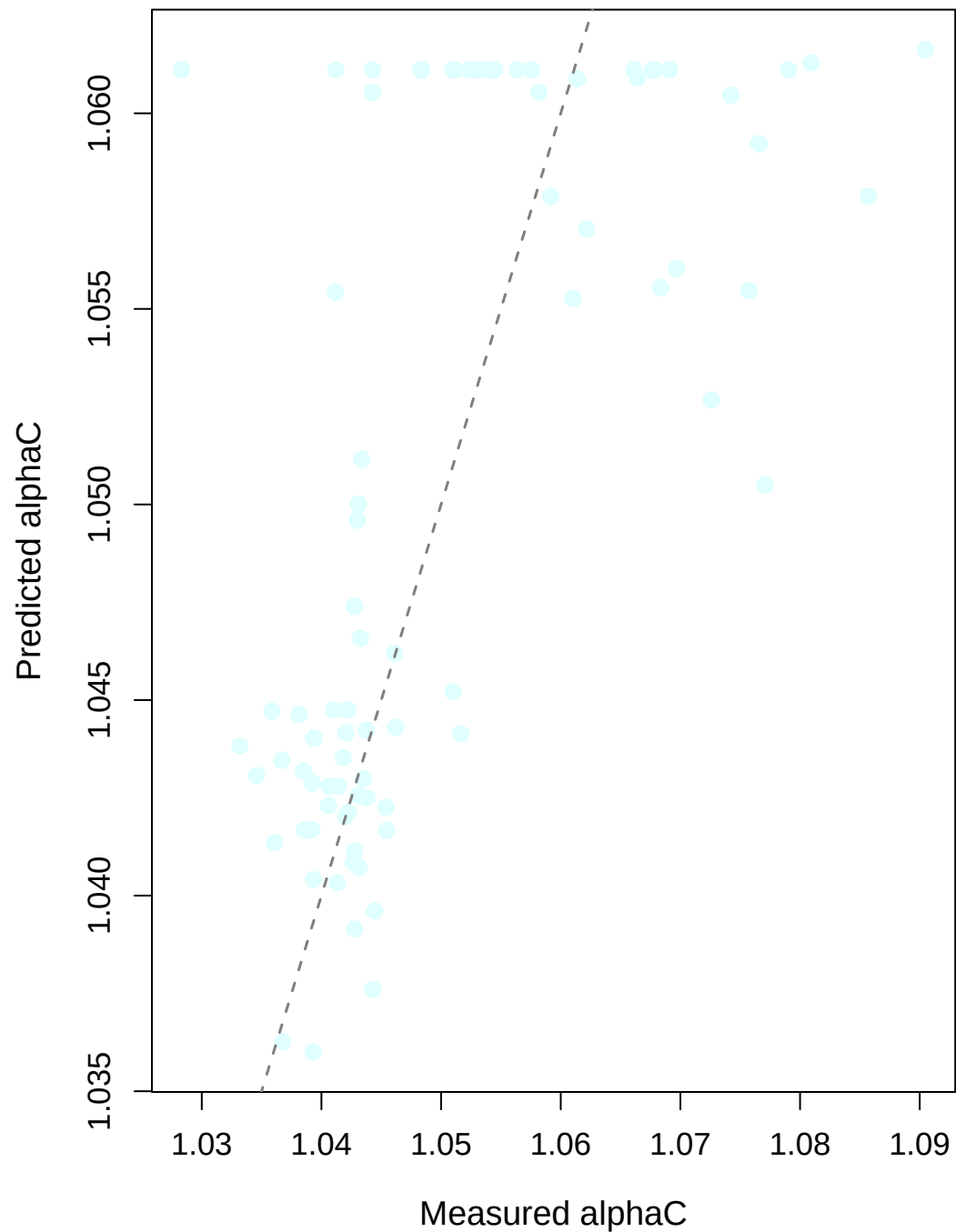
PLS LOO Performance (comp = 2, R^2 = 0.412 , RMSE = 0.010)
