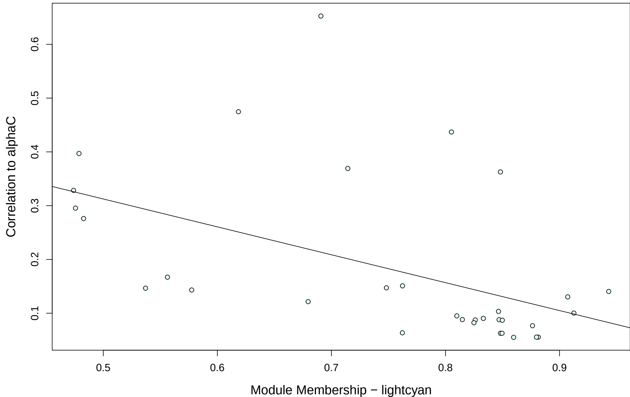
Module Membership vs. Trait Significance (Module: lightcyan | Trait: alphaC) cor=-0.5, p=0.003
