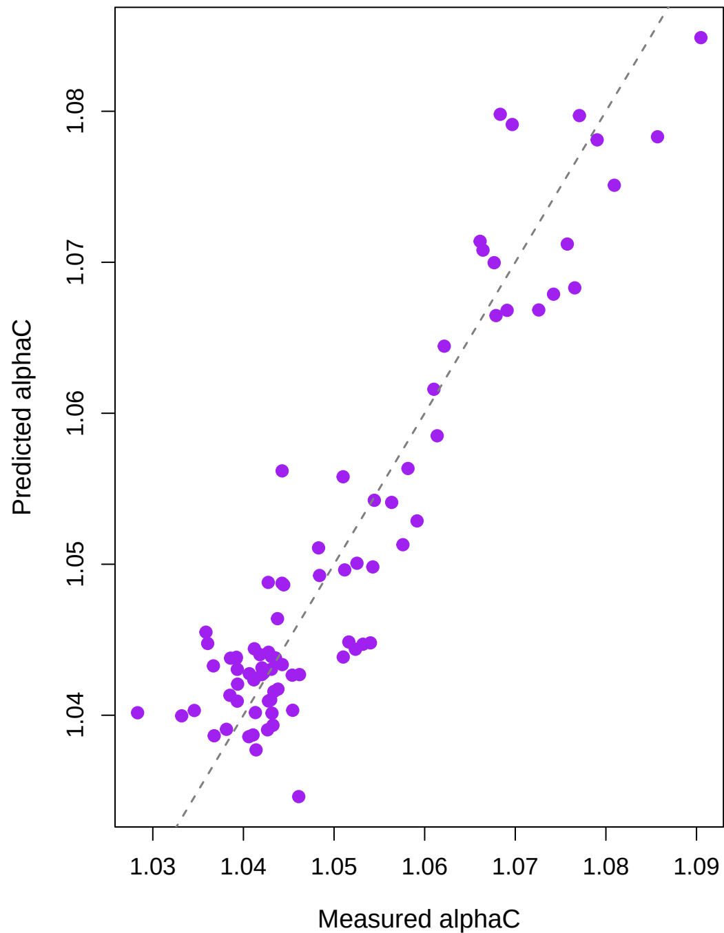
PLS LOO Performance (comp = 5, R^2 = 0.863 , RMSE = 0.005)
