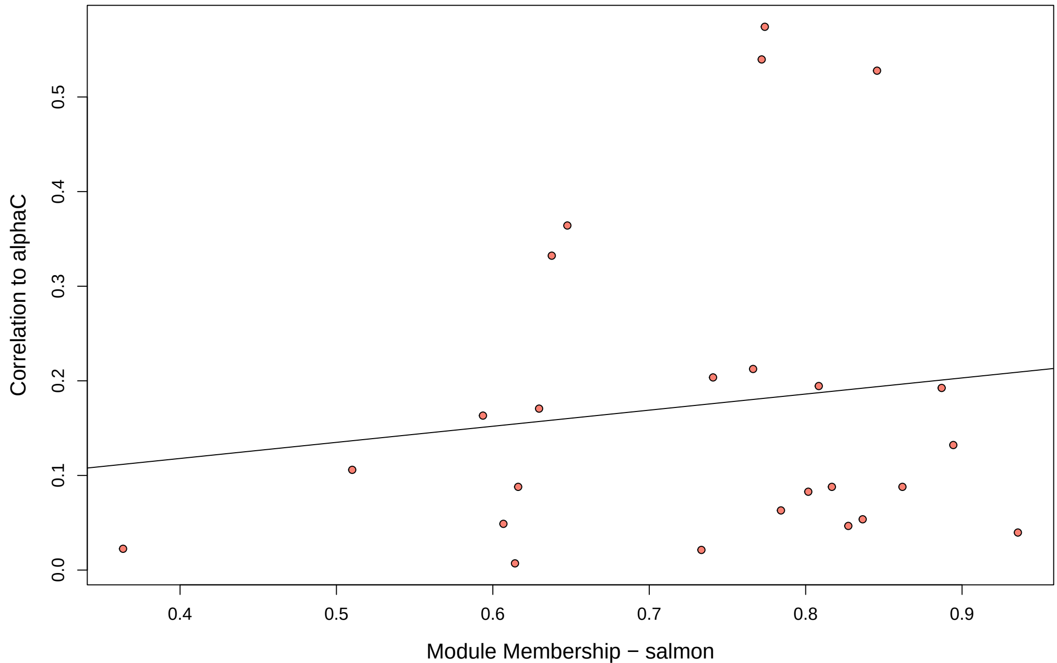
Module Membership vs. Trait Significance (Module: salmon | Trait: alphaC) cor=0.14, p=0.5
