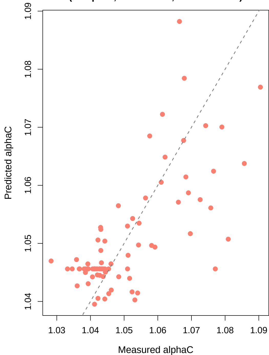
PLS LOO Performance (comp = 3, R^2 = 0.505 , RMSE = 0.010)
