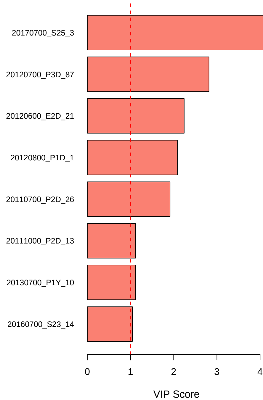
Predictors with VIP > 1 in Module: salmon (Predicting \alpha_C )
