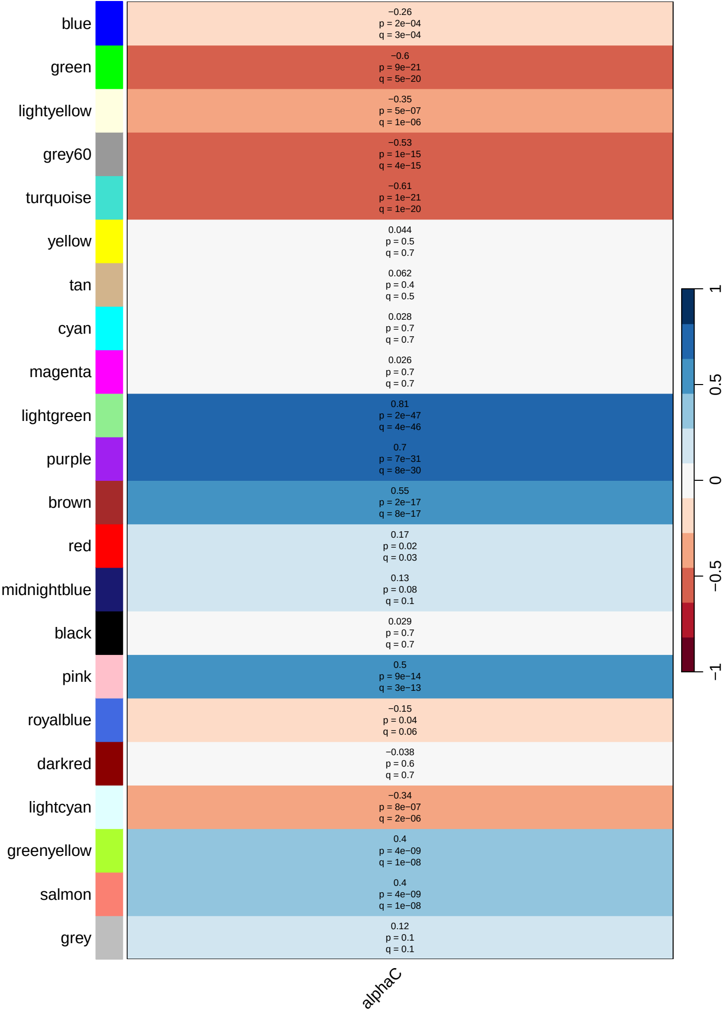
Module–trait relationships
