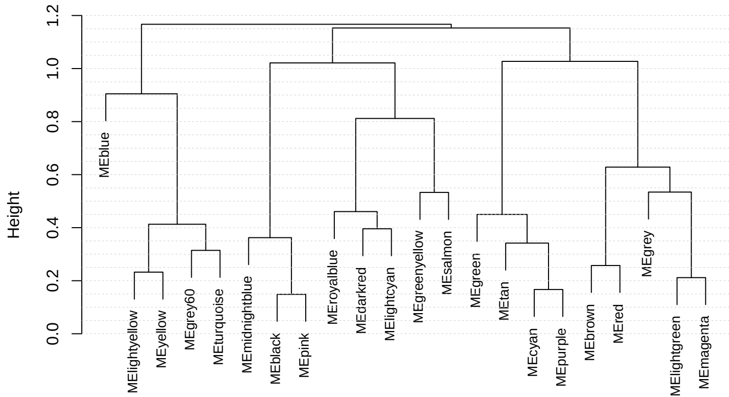
Unmerged Eigengene dendrogram (Before Merging)
