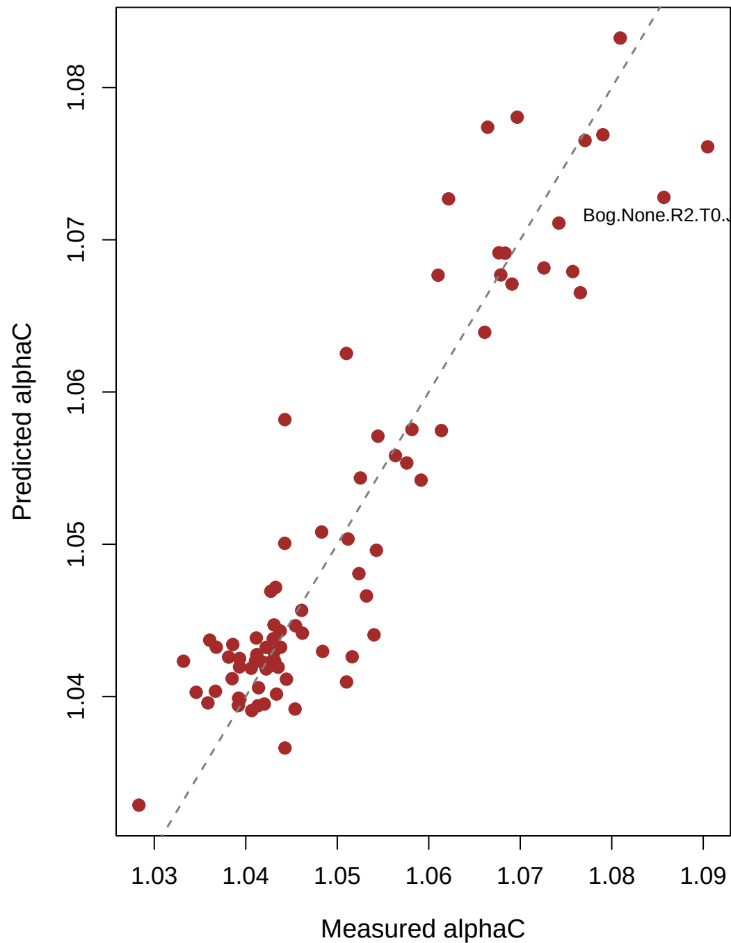
PLS LOO Performance (comp = 4, R^2 = 0.851 , RMSE = 0.005)
