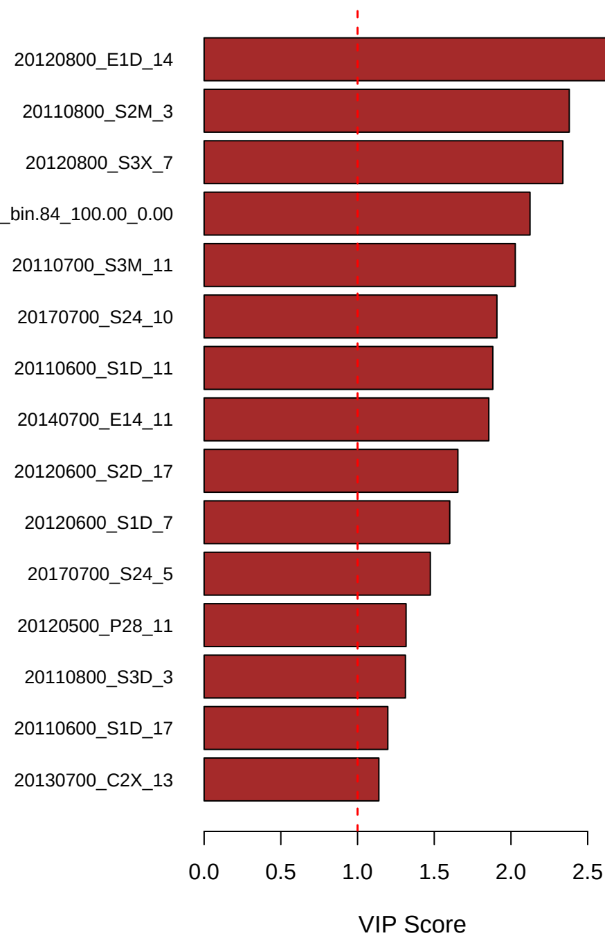
Predictors with VIP > 1 in Module: brown (Predicting \alpha_C )
