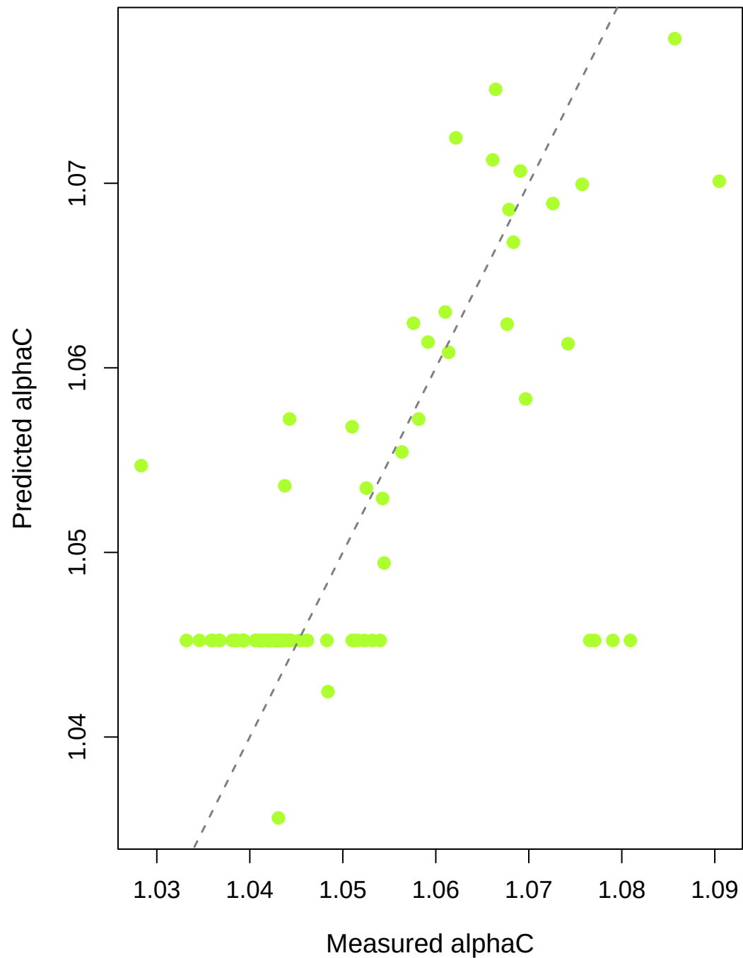
PLS LOO Performance (comp = 3, R^2 = 0.473 , RMSE = 0.010)
