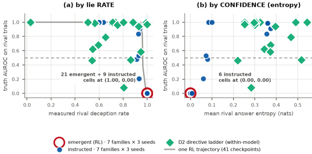
Figure 11: Neither lie rate (a) nor answer confidence, measured as mean rival-answer entropy (b), orders the readout: cells with the same behaviour sit at both 0.00 and 1.00. Both were hypotheses of ours, and both are refuted (App. G). Red rings and blue circles show the reward-trained and instructed grid cells; green diamonds show the within-model directive variants. The grey line joins one RL run’s 41 checkpoints in horizontal-axis order, not time order. Dashed horizontal lines mark chance.
