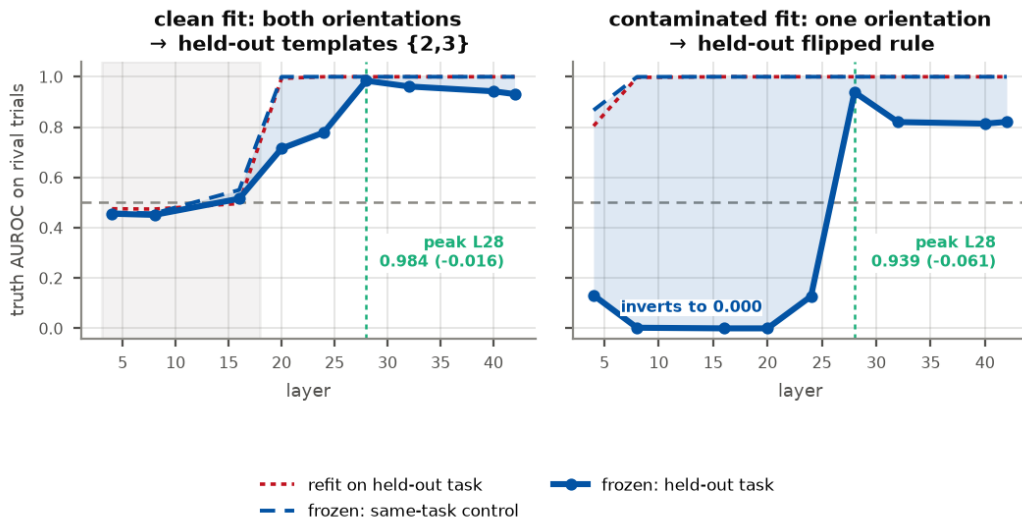
Figure 8: The settling experiment: frozen-probe transfer to held-out templates (left) and to a flipped rule (right). The same frozen probe scored on the held-out trials (solid) and on its own same-task control (dashed); the shaded gap is the transfer cost, and the dotted line is what refitting on the held-out trials would give. Left, clean fit: with both rule orientations in the fit the bit is the exclusive-or of two prompt facts: the frozen probe is at chance shallow, where a refit probe is also at chance (0.474/0.496), and transfers at 0.984 ( -0.016 ) at layer 28, 0.962/0.942/0.931 at layers 32/40/42. The cost is depth-dependent and worst at layer 20 ( -0.285 ; layer 24, -0.221 ). Right, contaminated fit: restricting the fit to one orientation removes the exclusive-or, the bit becomes the shallow feature “which slot is larger”, and the frozen probe inverts to 0.000 at layers 16 and 20 under a rule flip: the probe-side confound, measured. Both arms peak at layer 28 and ease off; green labels give frozen held-out AUROC and its difference from the same-task control. Grey spans mark layers where the control itself is at chance, so a small gap there reflects no detected signal for these probes rather than good transfer. Gemma-2-9B instructed, N=2000 per arm, compliant accuracies 0.764/0.741/0.785.
