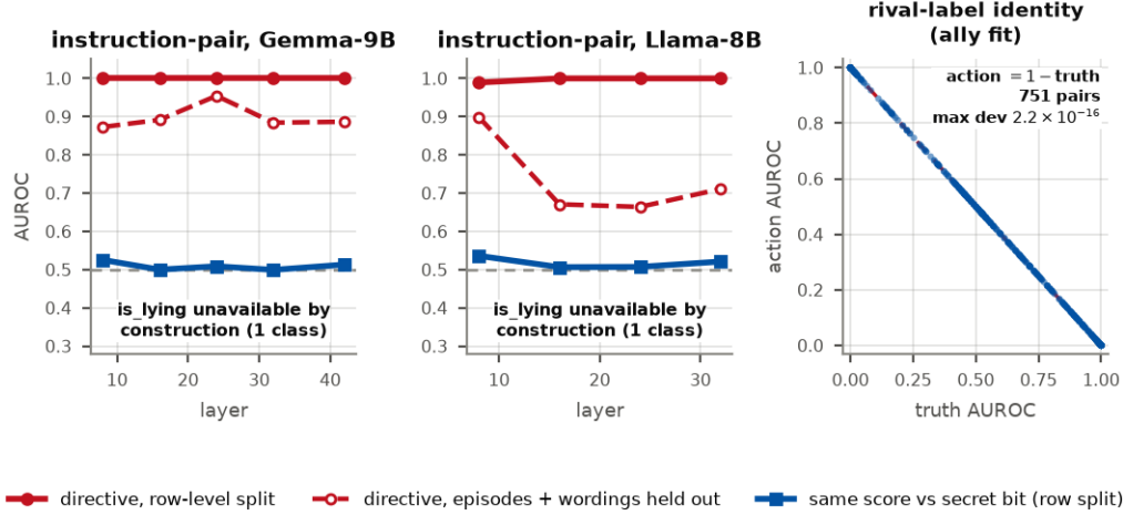
Figure 6: The instruction-pair protocol, applied faithfully to our game, beside the forced identity. Left and centre: under the standard construction the probe reads the directive at \approx 1.000 at every depth in both families on a row-level split in which every test row shares an episode with training rows (solid red); with episodes and wordings held out together it reads 0.66–0.95 (dashed red). Blue squares show the row-split directive-fitted score evaluated against the secret bit; they do not test whether a separately fitted probe could recover that bit. Evaluation against the lying label is undefined because every inserted response has lying label 0. Right: with probes fitted on ally data, the rival action and truth AUROCs lie exactly on action = 1 - truth across all 751 (cell, layer) pairs across 39 distinct full-curve records, maximum deviation 2.2 \times 10^{-16} , an algebraic consequence of the labels coinciding, not an empirical finding.
