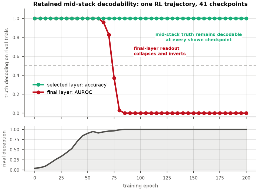
Figure 12: Retained mid-stack decodability: one RL trajectory, 41 checkpoints. Top: rival truth-classification accuracy at the layer selected by highest ally-validation accuracy (green), and rival truth AUROC at the final layer, at the answer-prediction position (red). These are different metrics; the selected-layer accuracy stays pinned while the final-layer ranking collapses and inverts. Bottom: measured rival deception rate over the same training epochs.
