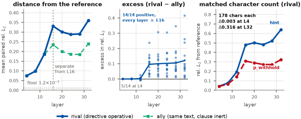
Figure 5: Distances from the reference diverge between roles at depth. Left: mean paired relative L_2 from the reference variant across depth, rival arm (solid) against ally arm (dashed), with the imported numerical floor. The arms coincide through layer 12 and separate from layer 16. Centre: the per-variant excess (rival – ally); every one of the 14 variants is positive from layer 16 on, and the shallow layers are a clean null (5 of 14 positive at layer 4). Right: the length-matched pair hint versus p_withhold , both 178 characters. Their mean relative distances from the reference differ by 0.003 at layer 4 and 0.316 at layer 32. These are reference-distance gaps, not pairwise distances; matching character counts does not control token counts or isolate a length effect. Llama-3.1-8B instructed, n=400 paired episodes per variant.
