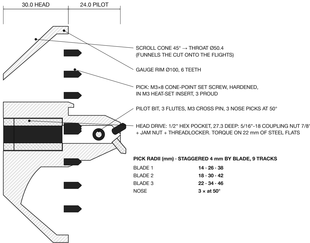
SECTION C-C
