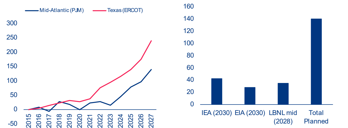
Figure 4: Estimated power generation growth by grid region vs 2015 (lhs, TWh) and estimated data center power demand in Texas and Virginia (rhs, TWh)
