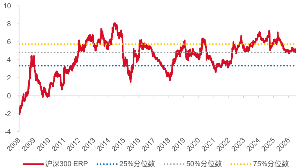
沪深300ERP
