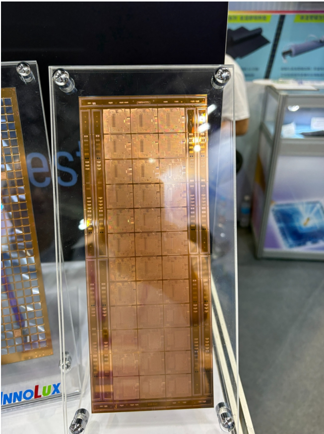
Figure 7: Innolux's chip-last FOPLP stripe – front end process by Innolux
