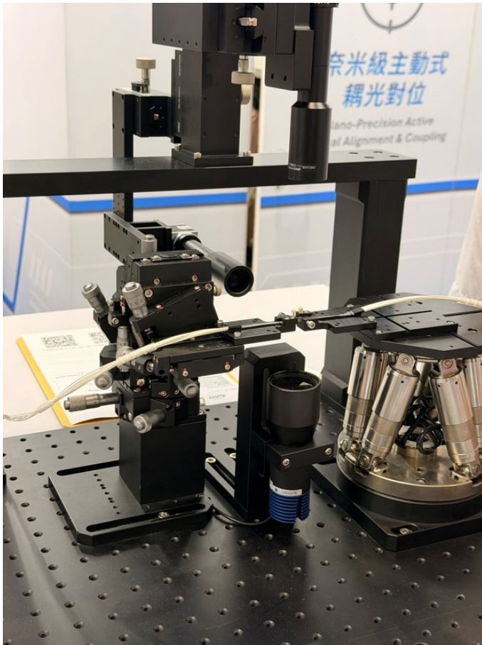
Exhibit 1: GMT (not covered) High-Precision Hexapod Platform could help for SiPh/CPO alignment
