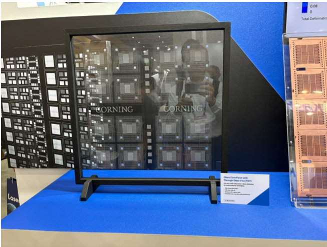
Figure 9: Corning's glass core panel with TGV
