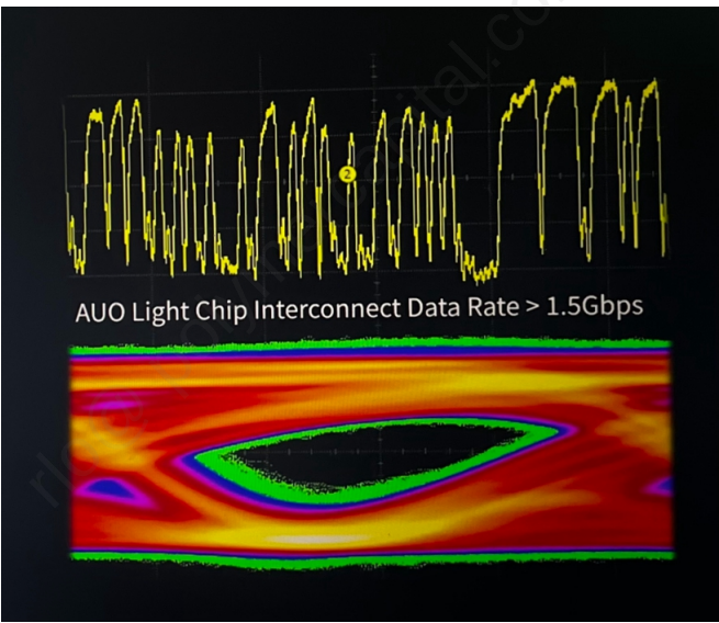
Figure 3: AUO demonstrated the open-eye diagram of its micoLED base solution
