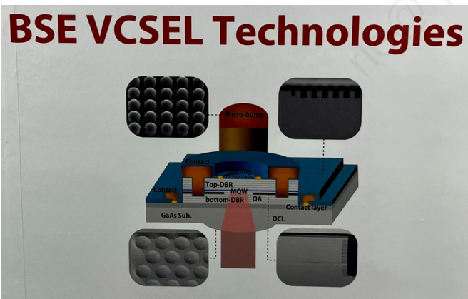
Figure 5: WIN Semi's BSE VCSEL Technologies
