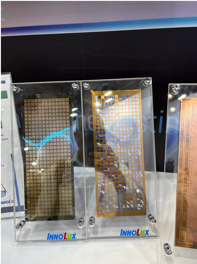
Figure 8: Innolux's chip-last FOPLP stripe – die attach and molding by OSAT customers
