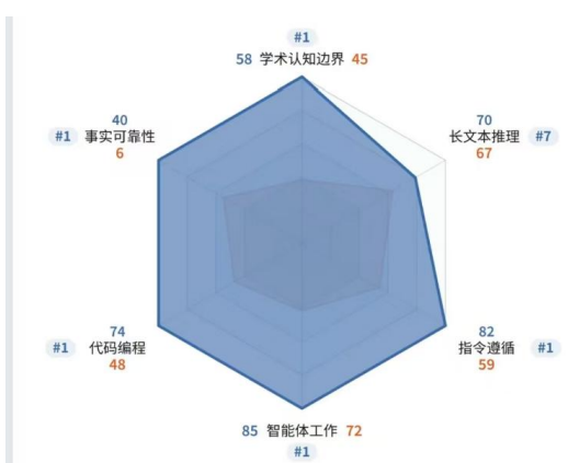
Claude Fable 5
