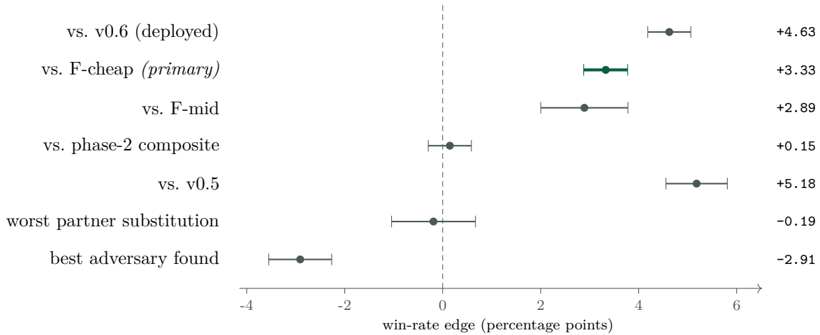
Figure 3: Principal comparisons for FishBot v0.7, pooled over both holdout banks with 95% deal-clustered bootstrap confidence intervals. Positive values favour FishBot v0.7. The registered primary comparison is highlighted. The bottom two rows place two robustness results on the same axis: the worst partner substitution of §11.5, and the most successful of the 8 adversarial searches of §11.8.
