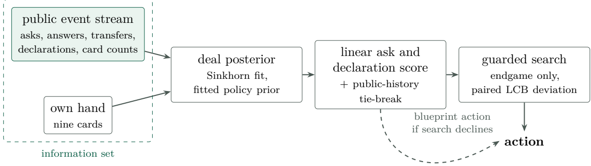
Figure 1: The information structure of a Fish seat and the FishBot v0.7 decision pipeline. A seat observes the public event stream and its own hand, and nothing else; there is no path from a policy to the deal or to another seat’s hand (§5.2). Because every card movement is public, that information set determines an exact posterior over the initial deal (§5). The deployed path does not construct it: it runs a cheaper approximate fit that starts from a policy prior and imposes the same constraints iteratively (§5.5). The search runs only in the endgame and departs from the blueprint’s choice only when a paired lower-confidence bound justifies it (§6.7).
