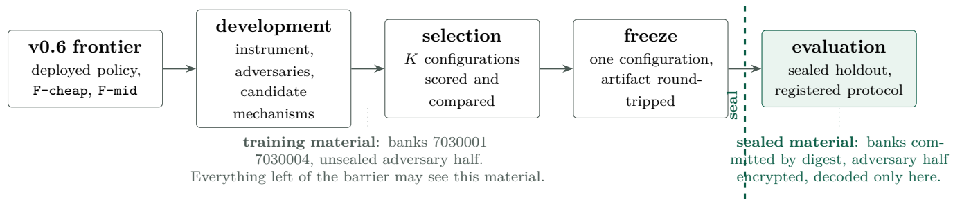
Figure 2: The development and evaluation protocol. Configurations were generated, scored and selected using training material only. Exactly one configuration was then frozen, and evaluated against material whose digests had been committed before any candidate existed, under a protocol registered in advance (§7.6). The seal is enforced by the engine rather than by convention: a run naming a sealed seed fails unless an explicit variable is set, which was set once and recorded.
