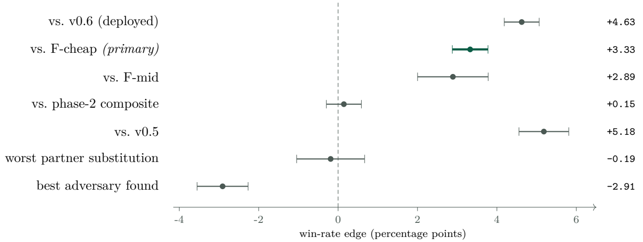
Figure 3: Principal comparisons for FishBot v0.7, pooled over both holdout banks with 95% deal-clustered bootstrap confidence intervals. Positive values favour FishBot v0.7. The registered primary comparison is highlighted. The bottom two rows place two robustness results on the same axis: the worst partner substitution of §11.5, and the most successful of the 8 adversarial searches of §11.8.
