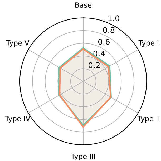
Recall
