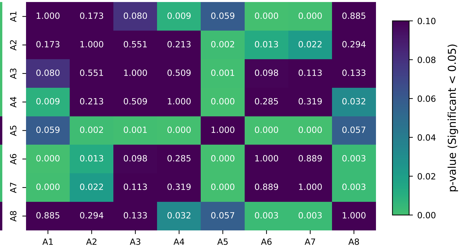
(b) Feed-Forward SNN
