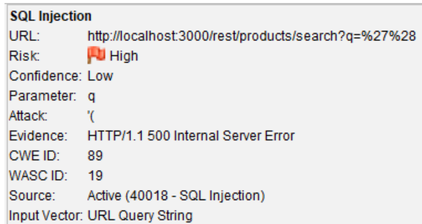
Figure 8: SQL Injection alert details raised by ZAP for /rest/products/search .
