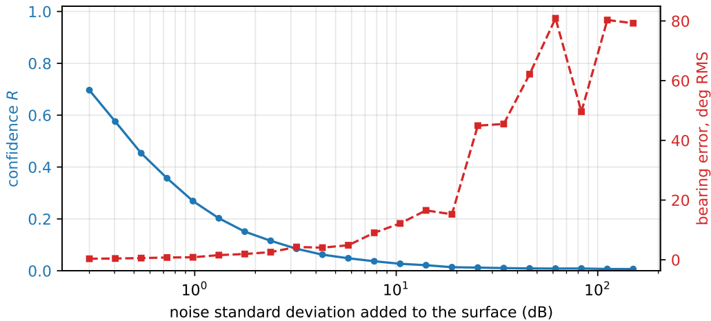
Figure 5: A clean planar surface at 45^\circ with increasing zero-mean noise. R has already fallen below 0.2 while the bearing is still within a couple of degrees. Treat a low R as a warning to look at the plot, not as an error bar.
