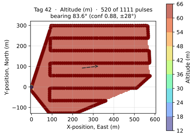
Figure 6: The third failure mode, and the reason the confidence is not a measure of correctness. This is the Day 5 flight with Property set to Altitude (m) : the surface is the aircraft’s own height profile, so the field agrees strongly ( R = 0.88 , the highest number in this guide) on a bearing of 83.6^\circ that has nothing whatever to do with the tag. A high R means the cells agree, not that you asked a sensible question.
