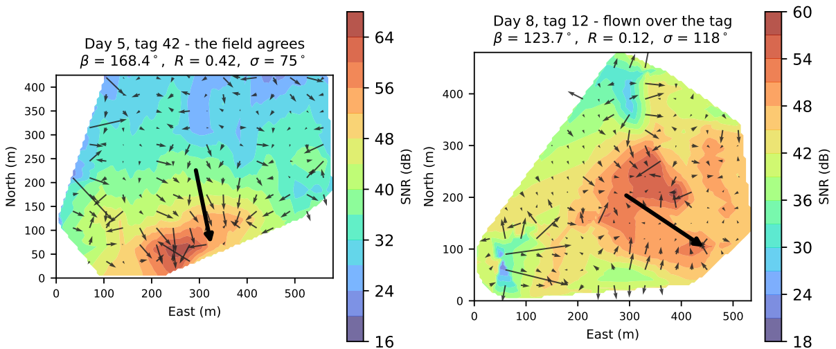
Figure 4: The gradient field the estimate is built from, on two real flights. Left: the arrows broadly agree and the resultant is meaningful. Right: the aircraft passed over the tag, so the gradients converge on an interior maximum and cancel; the resultant still has a direction but R = 0.12 says not to trust it. Both panels are computed by the application's own code.
