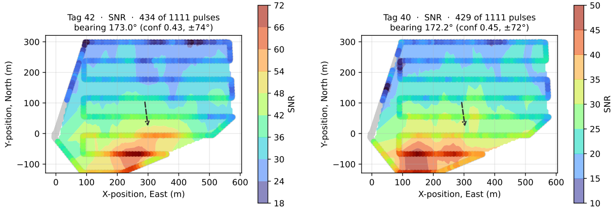
Figure 3: Day 5, tag 42 (left) and tag 40 (right) from the same flight, on the default time window: 434 and 429 pulses respectively. Grey dots are all 1111 pulses in the file, including the tags not selected and the takeoff and landing the window excludes; coloured dots are the selection; the filled surface is SNR interpolated over it. The two tags agree on a bearing to within a degree. Real output from the application.
