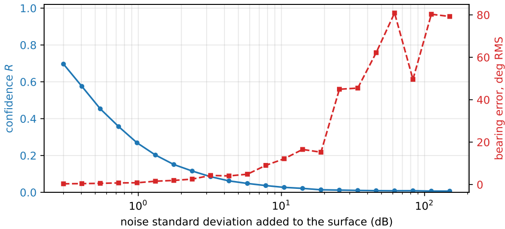
Figure 7: A clean planar surface at 45^\circ with increasing zero-mean noise. R has already fallen below 0.2 while the bearing is still within a couple of degrees. Treat a low R as a warning to look at the plot, not as an error bar.
