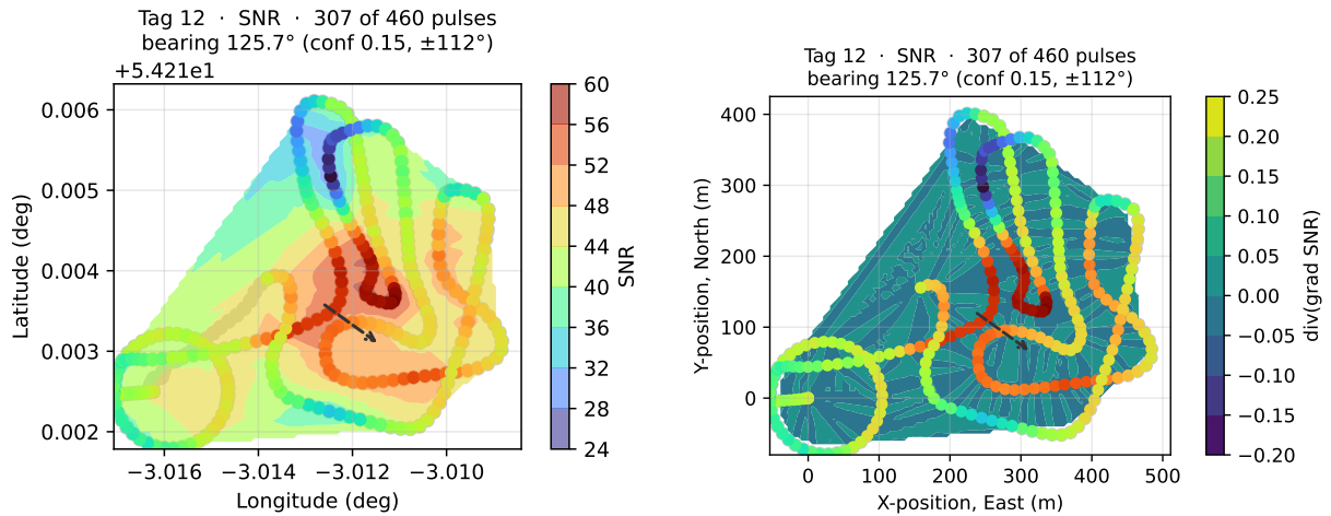
Figure 4: Day 8, tag 12. Left: the same data in Lon, Lat rather than x, y; the aspect ratio is corrected for latitude so the map is not stretched east–west. Right: Divergence mode, which shows where the gradient field converges — the dark region is where the surface peaks.
