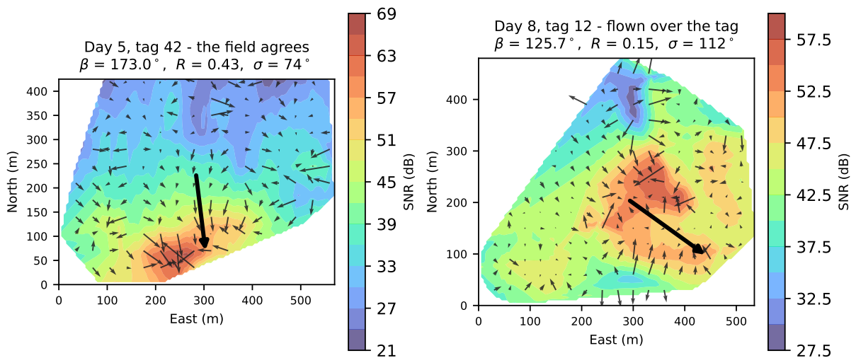
Figure 6: The gradient field the estimate is built from, on two real flights. Left: the arrows broadly agree and the resultant is meaningful. Right: the aircraft passed over the tag, so the gradients converge on an interior maximum and cancel; the resultant still has a direction but R = 0.15 says not to trust it. Both panels are computed by the application's own code.
