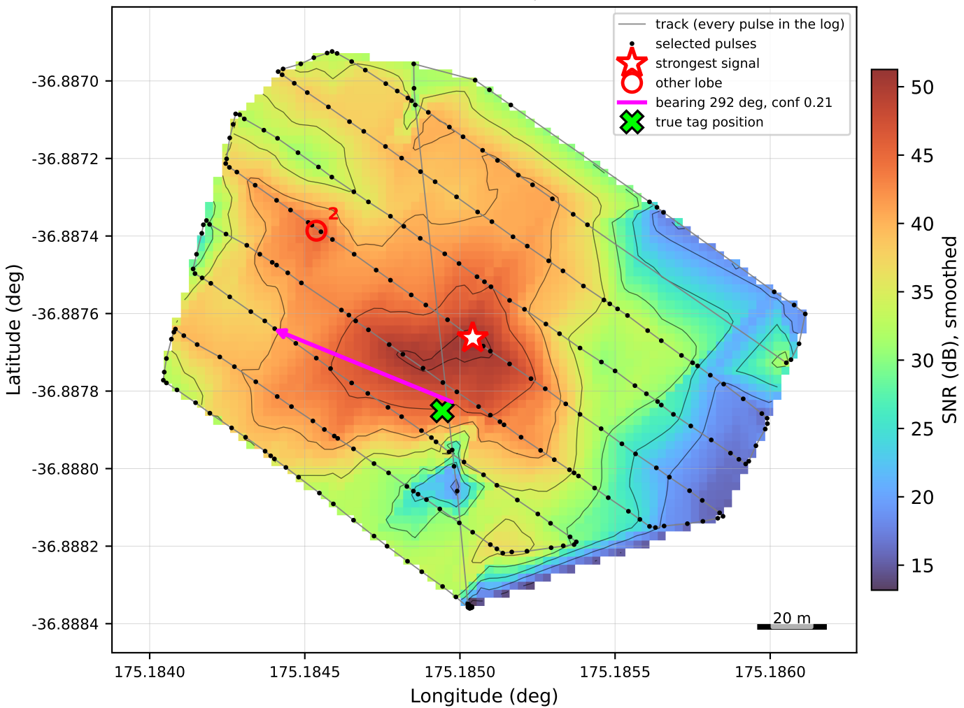
Tag 12 | 363 of 363 pulses | 0.0-10.0 min strongest signal -36.88766, 175.18504 | bearing 292 deg (conf 0.21)
