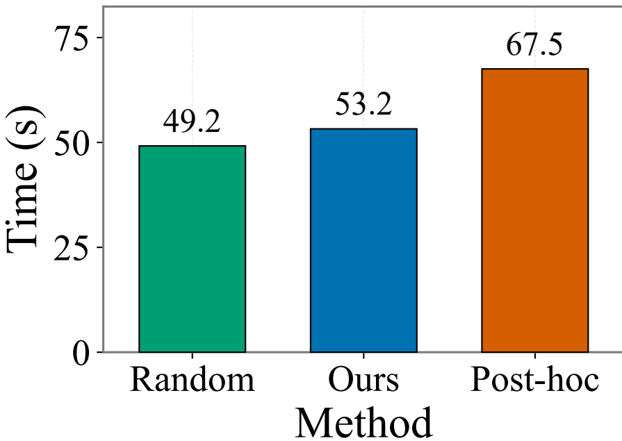
CIFAR-100 / ResNet
