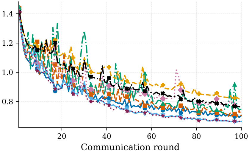
Training loss
