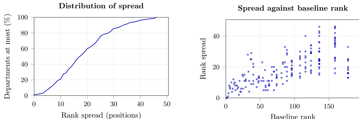
Figure 1: Rank spread across the 20-setting sweep, over 190 ranked U.S. departments. Stability is not a property of the ranking; it is a property of where in the ranking a department sits.
