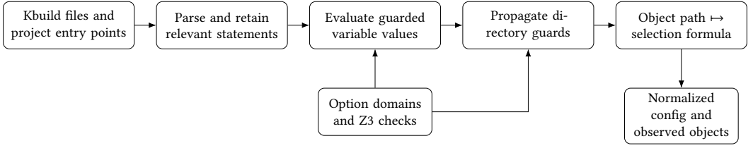
Fig. 1. The analysis produces Kbuild-local selection formulas before any concrete comparison. Configuration normalization and physical object inventory are separate validation inputs, not steps that make the symbolic conditions valid Kconfig assignments.
