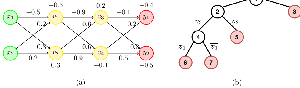
Figure 8.1: (a) A simple DNN (similar to Fig. 2.1), and (b) A proof tree produced by \text{BaB}_{\text{ProofGen}} . White nodes correspond to \text{BaB}_{\text{NNV}} neuron splitting. Red nodes correspond to leaf nodes where \text{BaB}_{\text{NNV}} determines infeasibility and prunes the branch.
