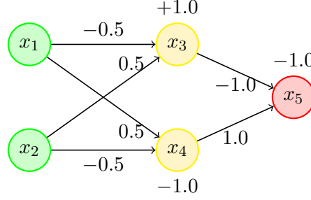
Figure 6.2: A simple network (similar to ??).
