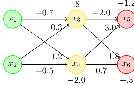
Figure 4.3: A simple network (similar to ??).
