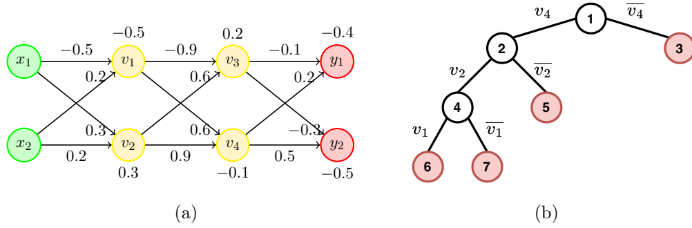
Figure 6.1: (a) A simple network (similar to ??), and (b) BaB search tree. White nodes correspond to \text{BaB}_{\text{NNV}} neuron splitting. Red nodes correspond to leaf nodes where \text{BaB}_{\text{NNV}} determines infeasibility and prunes the branch.
