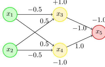
Figure 3.1: A simple network (similar to ??).
