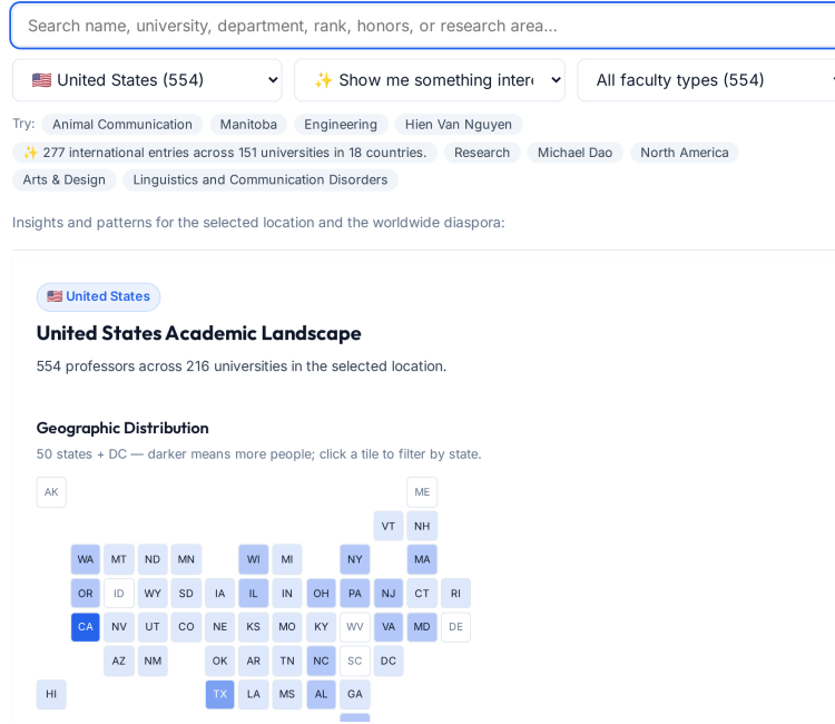
Figure 4: The runtime-computed “Show me something interesting” view for the United States subset, including the state-level choropleth grid ( src/state-grid.ts ); darker tiles indicate more records, and clicking a tile filters the roster to that state.
