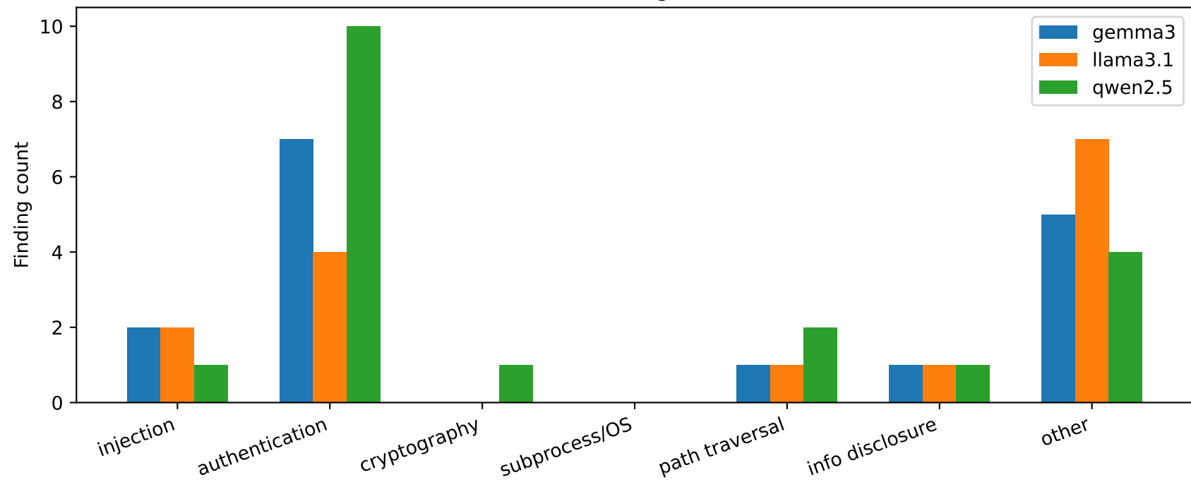
Snitch Issue Categories — Yum
