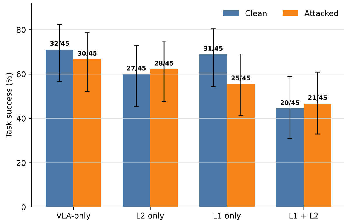
A. Task success (Wilson 95% CI)
