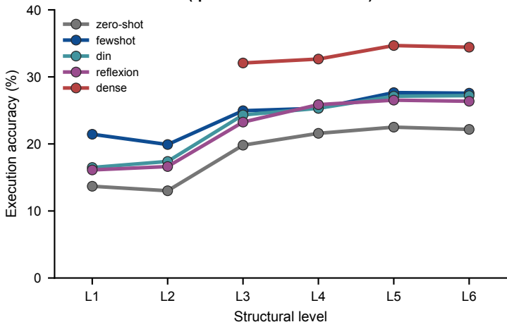
Prompting / self-correction methods by structural level (qwen2.5-coder-14b-local)
