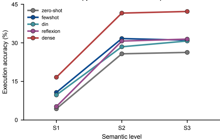
Prompting / self-correction methods by semantic level (qwen2.5-coder-14b-local)
