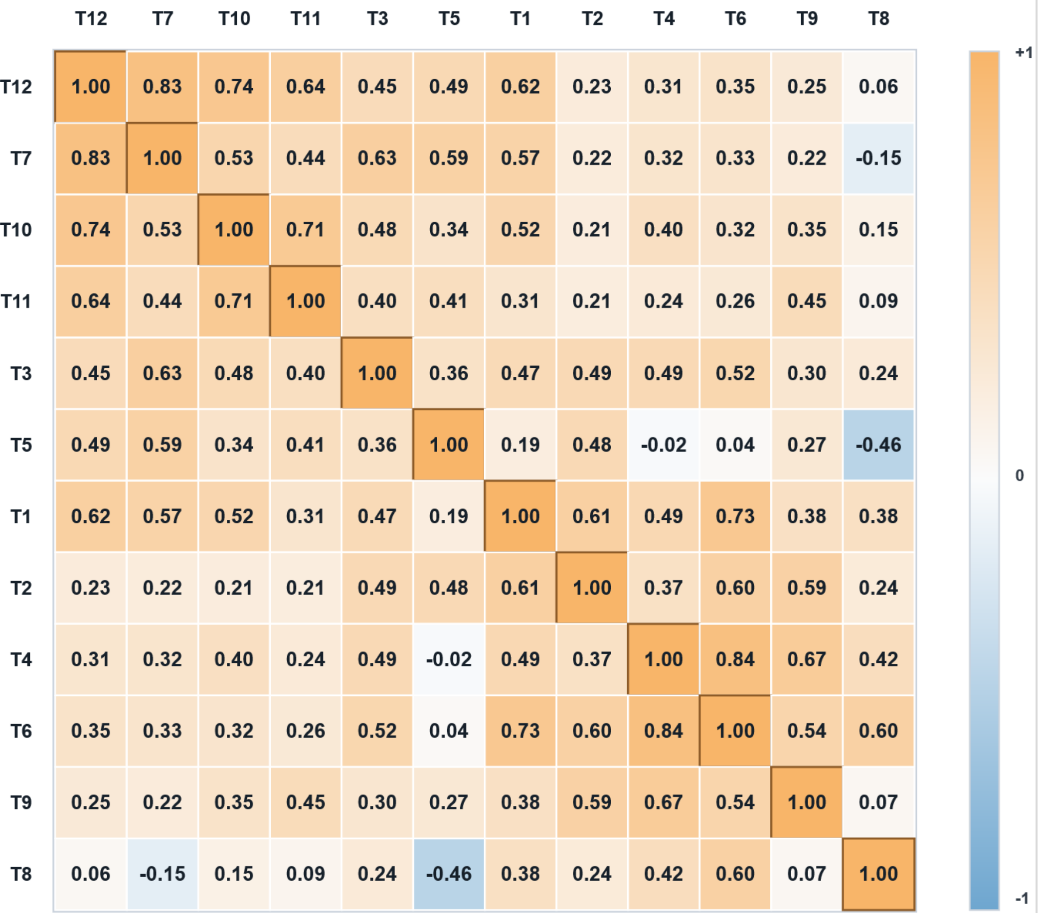
(a) Inter-task Correlation and Clustering Matrix
