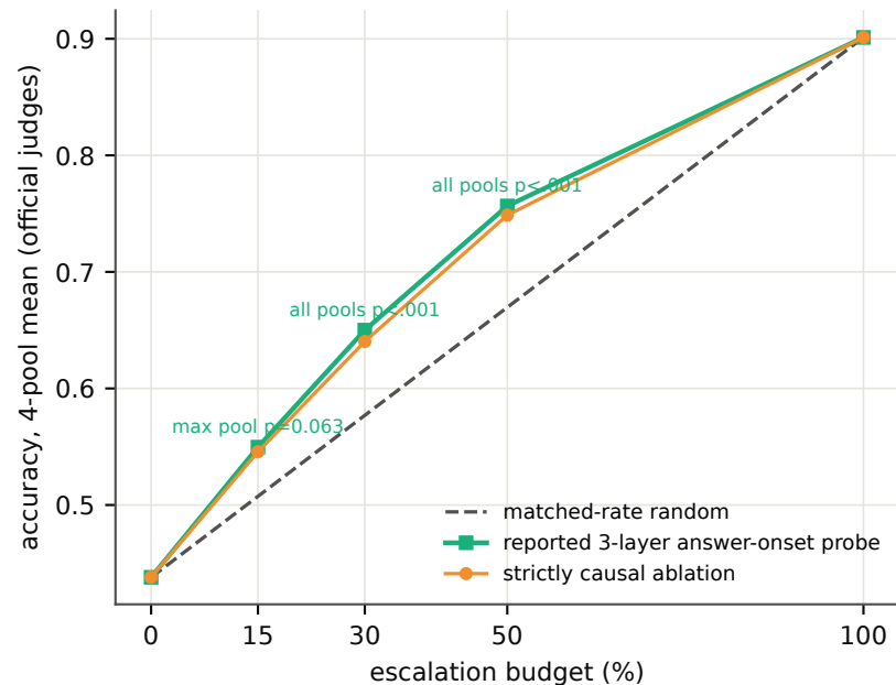
(b) Accuracy at fixed escalation budgets (official judges)
