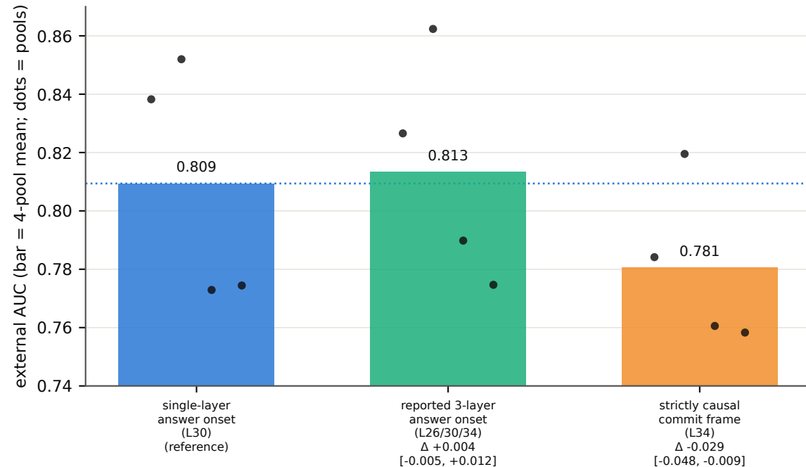
(a) External AUC by read point (pass-3; \Delta vs single-layer reference)
