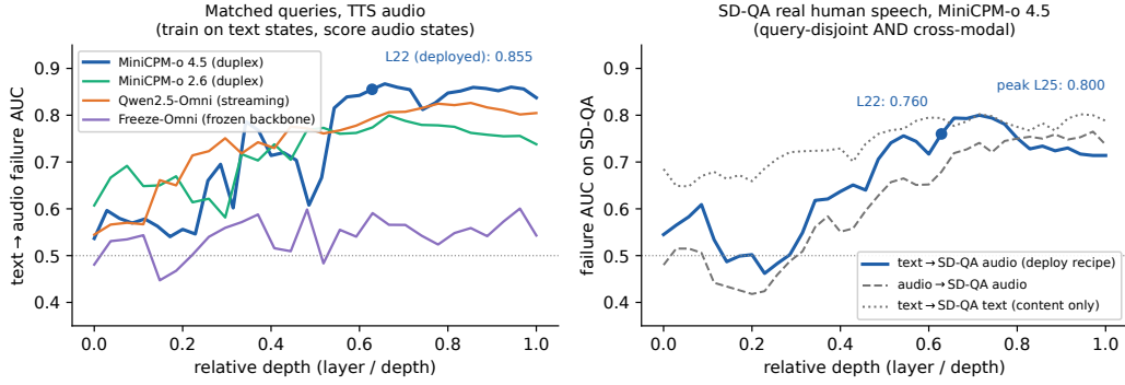
Figure 4: Text-trained failure probes transfer to unseen human speech. Left: matched-query modality transfer—probes fitted on text-input states are evaluated on TTS-audio states for the same 600 questions, across four models. MiniCPM-o 4.5 reaches 0.855 AUC at L22. Right: query-disjoint transfer—MiniCPM-o 4.5 probes fitted on the calibration pool are evaluated on 200 held-out SD-QA human recordings. The text-trained probe (blue) reaches 0.760 AUC at L22 and peaks at 0.800 at L25; gray curves show audio-trained and text-target references. These tests evaluate cross-modal transfer, complementing the text-only task-pool transfer in Figure 2. Depth is normalized by each model’s layer count.
