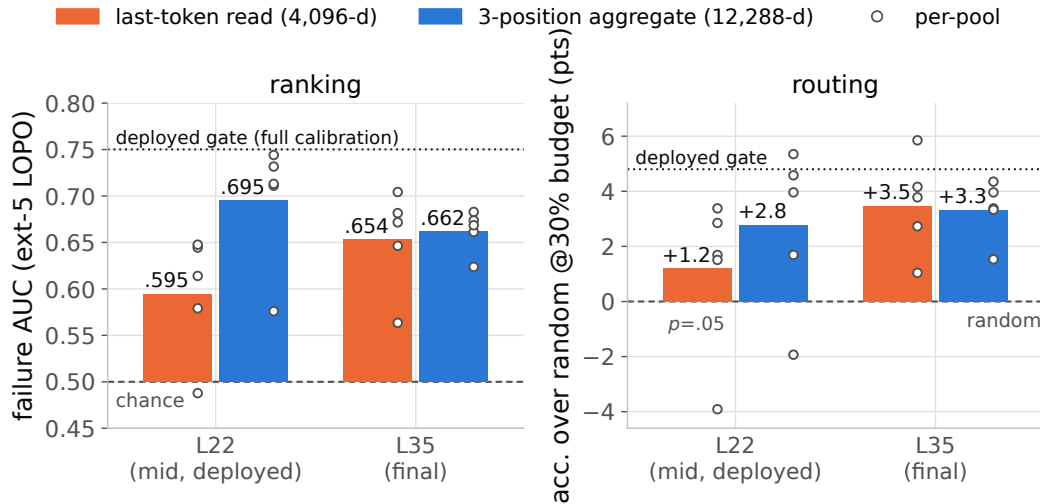
Figure 3: At the native commit point, position aggregation carries the read. Layer \times readout ablation, all four cells recomputed on one official-configuration batch (five external pools, LOPO; circles: held-out pools; dotted reference: the deployed gate, trained on the full calibration merge). Left: failure AUC. Right: accuracy over matched-random escalation at a 30% budget. The text-input mid-layer advantage (Figure 2) does not transfer to the audio commit read: single-token depth is flat-to-reversed, and the three-position aggregation restores the signal at L22 (+0.10 AUC) while adding almost nothing at the final layer.
