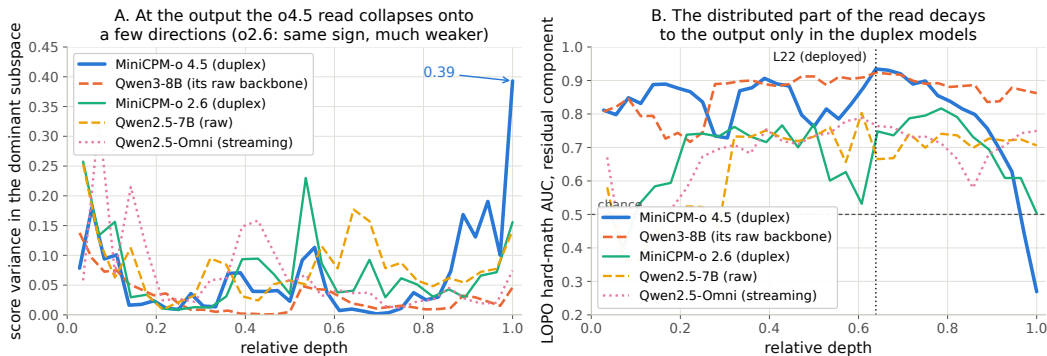
Figure 6: Non-destructive decomposition of the probe’s held-out score at every depth. Left: share of score variance carried by the layer’s five dominant probe directions. Right: transfer AUC of the residual (distributed) component, intact to the output on both raw backbones and on the omni-streaming control, decaying to inversion over the final layers of both duplex models.
