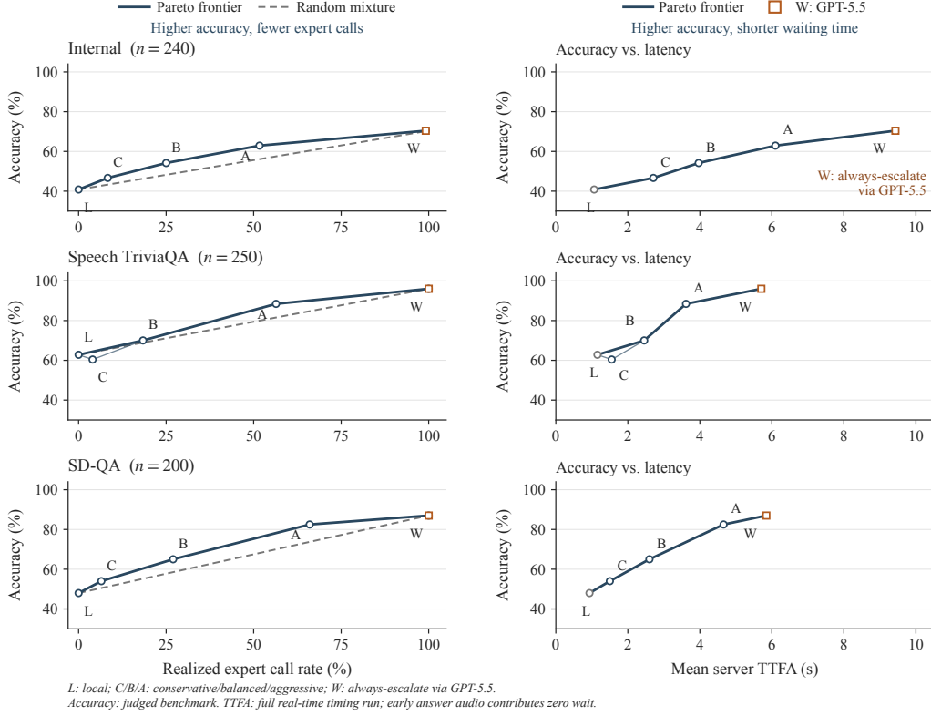
Figure 3: Accuracy-cost Pareto frontiers across routing policies. Left: accuracy versus expert call rate; dashed lines show random mixtures. Right: accuracy versus mean server TTFA. Thin solid lines connect all policy settings; thick lines connect nondominated policies. Always-escalate via GPT-5.5 (W) has the highest accuracy and latency on these pools; gated policies trade some accuracy for shorter waits. TriviaQA conservative is dominated by local. Accuracy retains the judged benchmark values; TTFA uses the full timing run (§4.1). Internal retains all 240 IDs with unit weights. L is local; C/B/A are conservative/balanced/aggressive.
