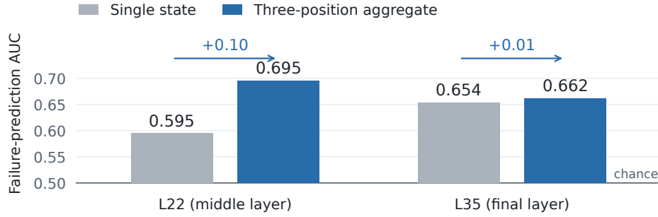
Figure 4: Aggregation improves failure prediction at L22. Mean AUC across five external pools under leave-one-pool-out evaluation on one native audio batch. Gray bars read the latest tail state; blue bars concatenate that state with the tail mean and input mean (§3.3). Arrows indicate the aggregation gain at each layer; the horizontal line marks chance AUC of 0.5.
