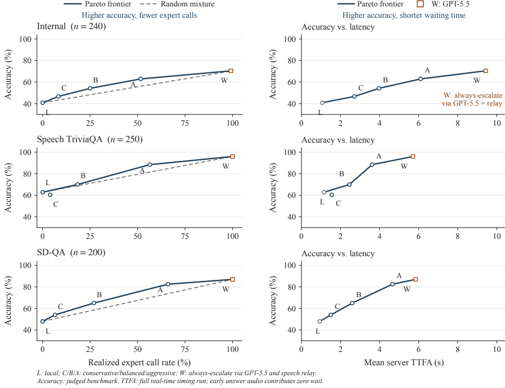
Figure 3: Accuracy–cost Pareto frontiers across routing policies. Left: accuracy versus expert call rate; dashed lines show random mixtures. Right: accuracy versus mean server TTFA. Solid lines connect nondominated policies under the reported metrics. Always-escalate via GPT-5.5 and speech relay (W) has the highest accuracy and latency on these pools; gated policies trade some accuracy for shorter waits. TriviaQA conservative is dominated by local. Accuracy retains the judged benchmark values; TTFA uses the full timing run (§4.1). Internal retains all 240 IDs with unit weights. L is local; C/B/A are conservative/balanced/aggressive.
