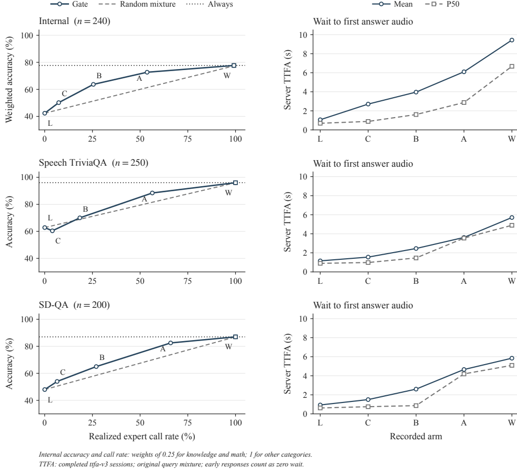
Figure 3: Accuracy and independently measured TTFA on three pools. Left: answer-content accuracy against expert call rate. Internal uses post-hoc weights of 0.25 for knowledge/math and 1 for other categories in both coordinates, retaining all 240 queries. Table 1 retains original query weights; external curves are unweighted. C/B/A denote conservative/balanced/aggressive. The dashed line follows the table’s random-mixture convention (§4.1); the horizontal reference is the measured always arm, not an oracle bound. Right: mean and P50 server TTFA from completed sessions in the independent ttfa-v3 run, with original query weights. TTFA is the nonnegative wait after input end until first answer PCM; early answers have zero wait. L/W denote local/always. Each query has one attempt per arm; candidate/stall audio and client playback are excluded. Timing-session answers are unjudged and do not establish the accuracy on the left. Internal counts and tails appear in Table 10; Table 1 covers all four external English speech-QA pools evaluated here.
