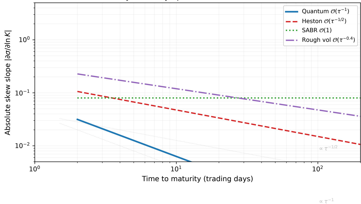
Short-Maturity Skew Asymptotics: Quantum vs Classical Models
