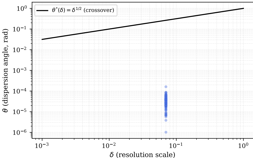
Crossover curve and n = 130 events
