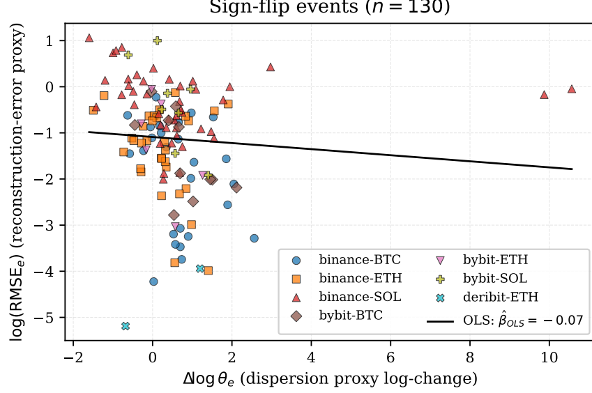
Figure 1: Log-log scatter of the reconstruction-error proxy against \Delta \log \theta across n = 130 sign-flip events; solid line: OLS fit ( \hat{\beta}_{OLS} = -0.07 ).
