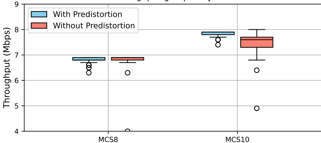
Throughput grouped by MCS
