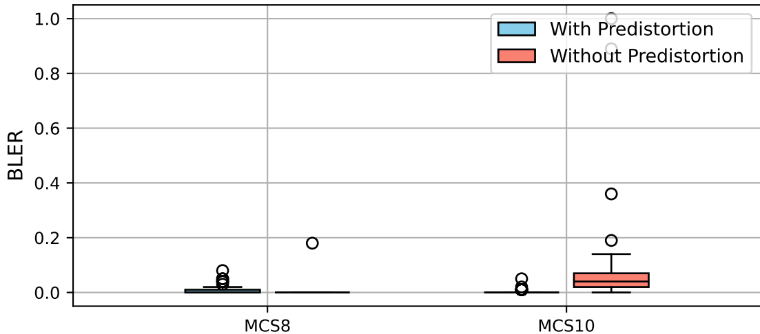
BLER grouped by MCS
